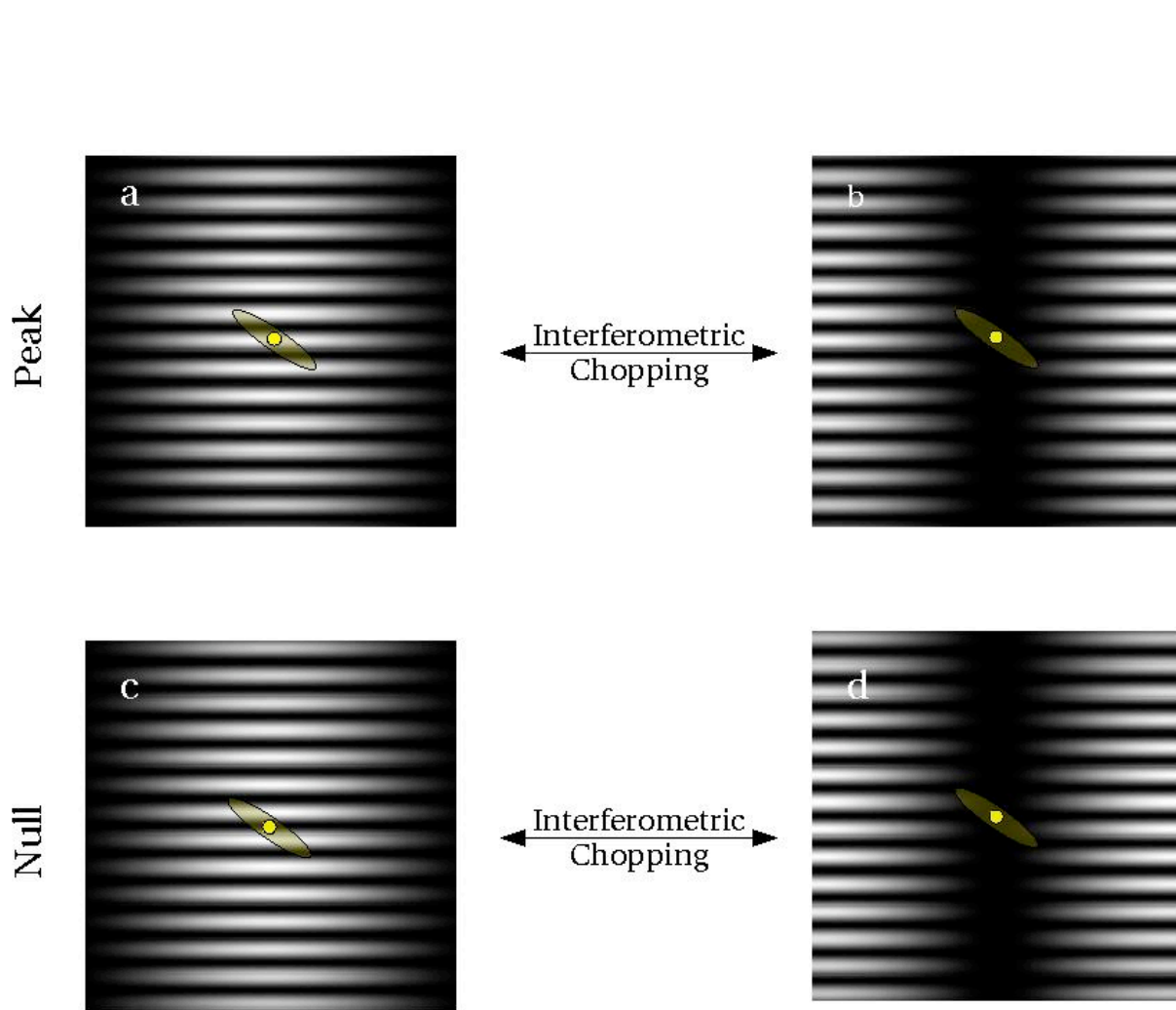
Figure 2. Fringes for a four-baseline nuller configuration in which the nulling is done on a pair of parallel long baselines. The short baseline produces a perpendicular set of broad fringes across the primary beam. Their phase is modulated at a rate fast enough to “chop out” the variations in the thermal background, a process we refer to as interferometric chopping . A schematic star+disk system is shown to illustrate the effect of the various fringe phases. The star is smaller than the spacing of the long-baseline fringes, while the size of the disk is intermediate between the spacings of the long and short baseline fringes. Figs 2a and 2b illustrate the measurement of the light from the central star, which is modulated by the movement of the short-baseline fringe. Figs 2c and 2d show the corresponding measurement of the disk, whose faint light is significant only because the starlight is suppressed by central null of the long-baseline fringe.
